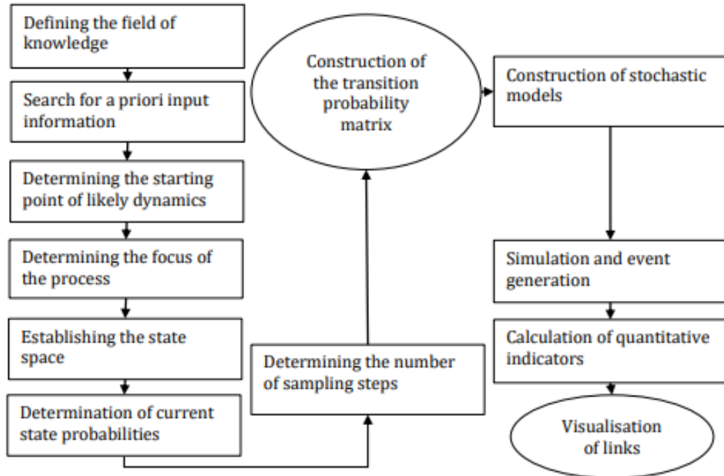
Figure 1: Conceptual model of probabilistic dynamics of innovation
