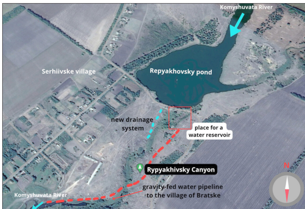
Fig. 3. The planned location of the water storage reservoir in the Komyshuvata River valley
