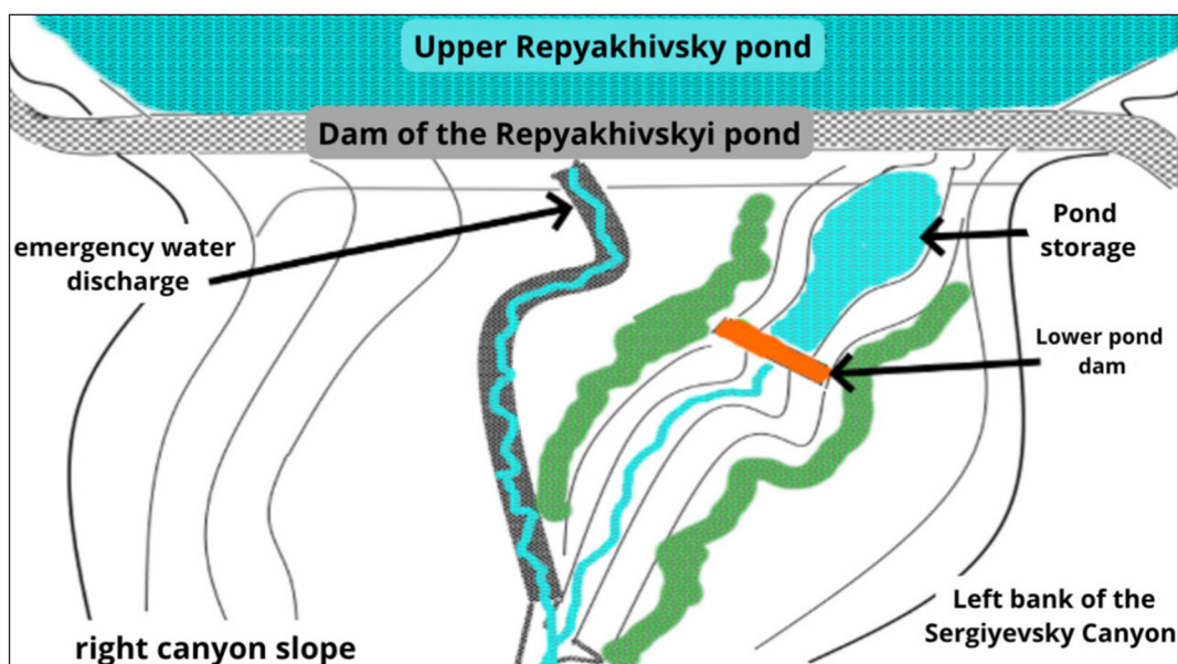
Fig. 6. The upper and lower ponds and their spillways within Serhiyivka Canyon
