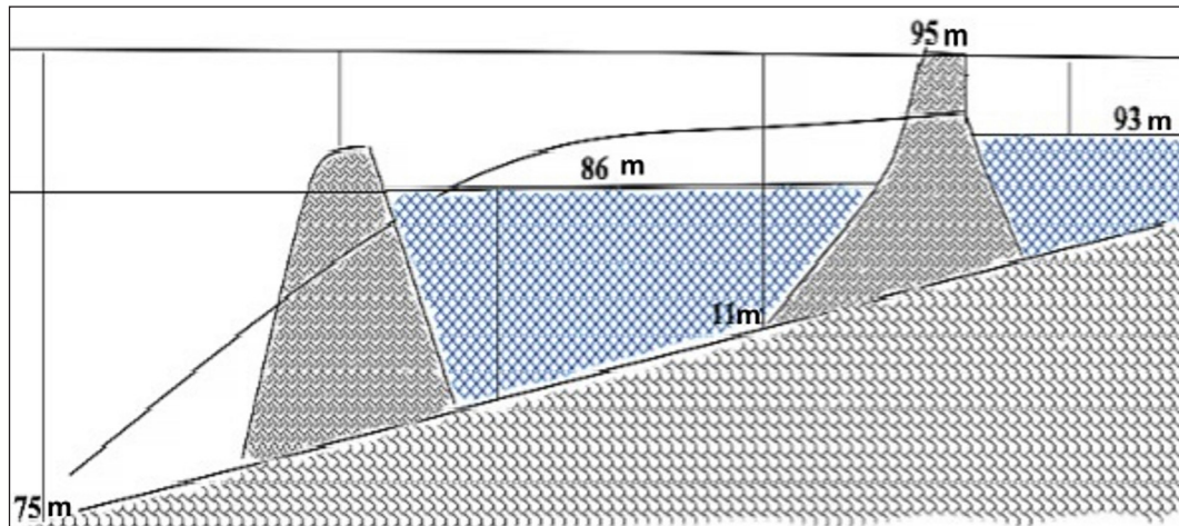
Fig. 5. Heights and profile of the channel and dam of the existing Repyakhivske pond along with the proposed dam of the storage reservoir, view from the left bank of the Komyshevata River
