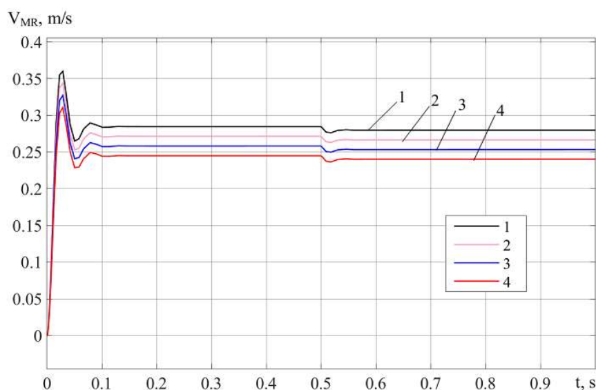
Fig. 6. Change in the MR's linear speed at the following modulus difference in the DCM supply voltages \Delta U_{12} : 1 – \Delta U_{12} = 0 V; 2 – \Delta U_{12} = 20 V; 3 – \Delta U_{12} = 40 V; 4 – \Delta U_{12} = 60 V
