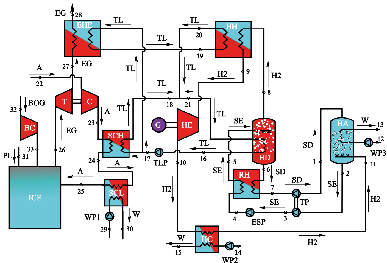
Figure 1. The physical structure of the waste heat recovery metal hydride unit
