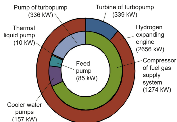
Figure 2. Components of mechanical energy of the disposal metal hydride unit
