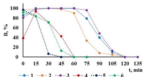
Fig. 8. Dependence of current efficiency of reduced cadmium on duration of electrolysis at current strength of 1 A (1, 2, 3) and of 2.5 (4, 5, 6) of the solution, containing ions of zinc, cadmium and sulfuric acid in concentrations, mg-equiv./dm 3 : 1, 4 – 399, 381, 624; 2, 5 – 399, 381, 259; 3, 6 – 400, 402, 0
