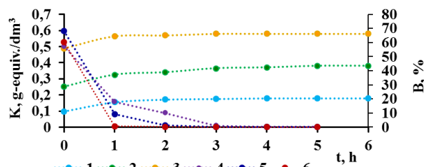
Fig. 2. Dependence of acidic solution (1; 2; 3) and current efficiency of metallic cadmium (4; 5; 6) on duration of electrolysis of acidic solution of cadmium sulfate at voltage of 5 V in single-chamber electrolyser ( V=0.1 dm 3 ) at initial cadmium concentrations (mg/dm 3 ) and sulfuric acid concentrations (mg-equiv./dm 3 ): 1, 4 – 4,721, 98; 2, 5 – 4,721, 250; 3, 6 – 5,508, 490
