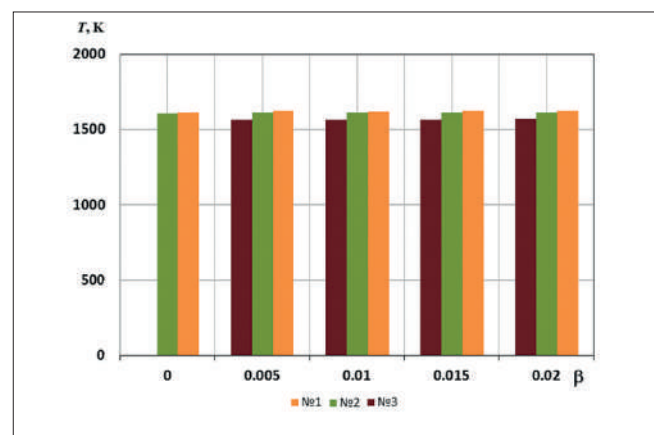
Fig. 6. Dependencies of temperatures in the outlet section of the flame tube on the amount of additives of plasma-chemical products for modes 1-3
