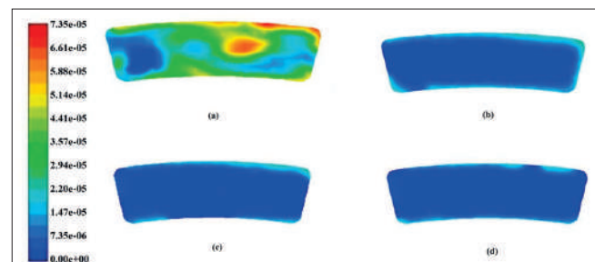
Fig. 5. Distribution of carbon monoxide concentrations at outlet section for the first mode of fuel supply: a - basic version without additions of plasma-chemical products; b - \beta = 0.005 ; c - \beta = 0.01 ; d - \beta = 0.02
