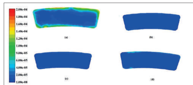
Fig. 4. Distribution of carbon monoxide concentrations at outlet section for the third mode of fuel supply: a - basic version without additions of plasma-chemical products; b - \beta = 0.005 ; c - \beta = 0.01 ; d - \beta = 0.02
