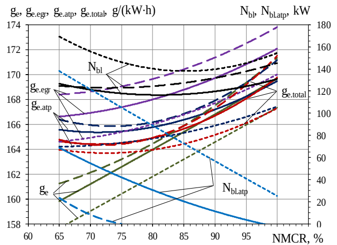
Figure 7 – Dependences of specific fuel consumption change for an engine without recirculation g_e , specific fuel consumption for an engine with recirculation g_{e,egr} , specific fuel consumption for an engine with recirculation and ATP g_{e,atp} , specific fuel consumption for an engine with recirculation, ATP and taking into account the reduction in load to the fan (EGR blower) g_{e,total} , recirculation fan power N_{bl} , recirculation fan power with ATP N_{bl,atp} from the load on the engine NMCR:
