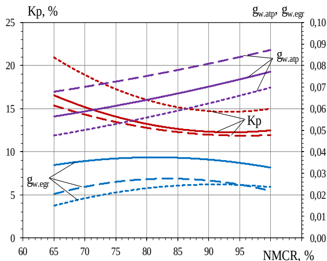
Figure 6 – Dependences of recirculation coefficient change K_p , relative consumption of water for injection in the ATP g_{w.atp} and in the scrubber g_{w.egr} from the load on the engine NMCR:
