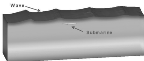
Fig. 6. Wave simulation by means of CFD tools (Flow-3D): a — dimensions of domain (in meters); b — fine meshes in Mesh Block2; c — generated wave and position of submarine
