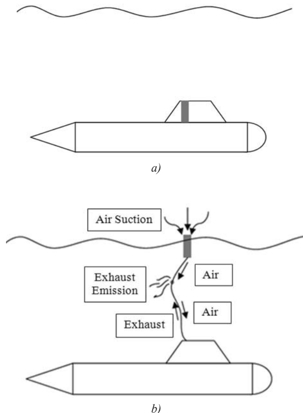
Fig. 4. Schematic of the Moon-Korol snorting system:
