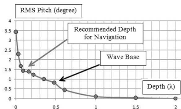
Fig.7. Gradient of RMS pitch versus submergence depth of a submarine
