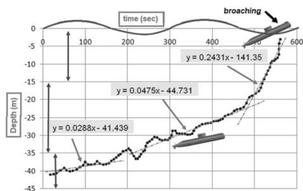
Fig. 12. Depth change due to the suction force from surface waves. Initial depth: 40 m, speed: 5 knots, regular waves height: 2.5 m, period: 8 sec, wave length: 103 m
