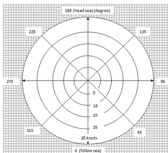
Fig. 10. SOE diagram for the pitch angle (limit value of 2.5 degree): submarine at snorting condition, JONSWAP spectrum, significant wave height of 2 m
