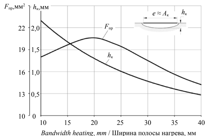
Fig. 3. Dependence of the depth h_k and penetration area F_{\text{пр}} on the width of the band of heating with the mobile source
