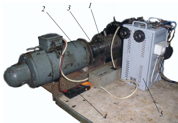
Fig. 1. Experimental bench for determining the power of mechanical losses of a prototype rotary piston engine 12 RPD 4.4/1.75 with a cam-articulated movement mechanism: 1 – rotary piston engine 12 RPD 4.4/1.75; 2 – DC electric motor 2PB-132MG; 3 – sleeve-finger coupling; 4 – digital multimeter PROTESTER M266C; 5 – autotransformer AOSN-20-220-75 UHL4
