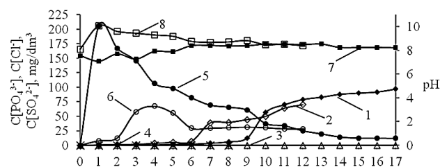
Fig. 4. Dependence of the concentration of phosphates (1; 2), sulphates (3; 4), chlorides (5; 6), pH of the medium (7; 8) on the volume of tap water ( \text{Hardness}=3.1 \text{ mg-equiv/dm}^3 ; \text{Alky}=4.9 \text{ mg-equiv/dm}^3 ; C(\text{PO}_4^{3-}) , \text{mg/dm}^3 : 105 (1; 3; 5; 7), 83 (2; 4; 6; 8); C(\text{Cl}^-) , \text{mg/dm}^3 : 12.07 (1; 3; 5; 7), 28.4 (2; 4; 6; 8); C(\text{SO}_4^{2-}) , \text{mg/dm}^3 : 36.7 (1; 3; 5; 7), 57 (2; 4; 6; 8)) passed through the anionite AV-17-8 in the Cl - (1; 3; 5; 7) and OH - (2; 4; 6; 8) form ( V_i=20 \text{ cm}^3 ) ( \text{FDEC}_1=1480 \text{ mg-equiv/dm}^3 ; \text{DEC}_{1\text{gap}}=689 \text{ mg-equiv/dm}^3 ; \text{FDEC}_2=930 \text{ mg-equiv/dm}^3 ; \text{DEC}_{2\text{gap}}=262 \text{ mg-equiv/dm}^3 ; \text{DEC}_{3\text{gap}}=646 \text{ mg-equiv/dm}^3 ; \text{DEC}_{4\text{gap}}=713 \text{ mg-equiv/dm}^3 )
