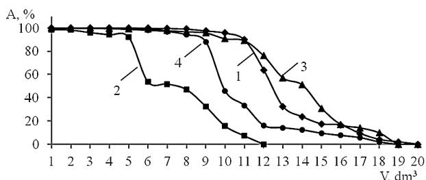
Fig. 5. Dependence of the degree of removal of phosphates on the anionite AV-17-8 ( V_i=20 cm 3 ) in the OH - (1; 2) and Cl - (3 and 4) form from the model solutions ( C(\text{PO}_4^{3-}) , mg/dm 3 : 97 (1), 92 (3)) and tap water ( C(\text{PO}_4^{3-}) , mg/dm 3 : 83 (2), 105 (4)) on the volume of the filtered solution
