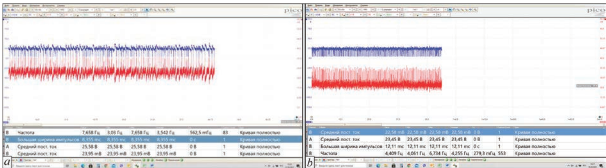
Figure 3. Oscillogram of welding process: a — conventional technology; b — improved technology
