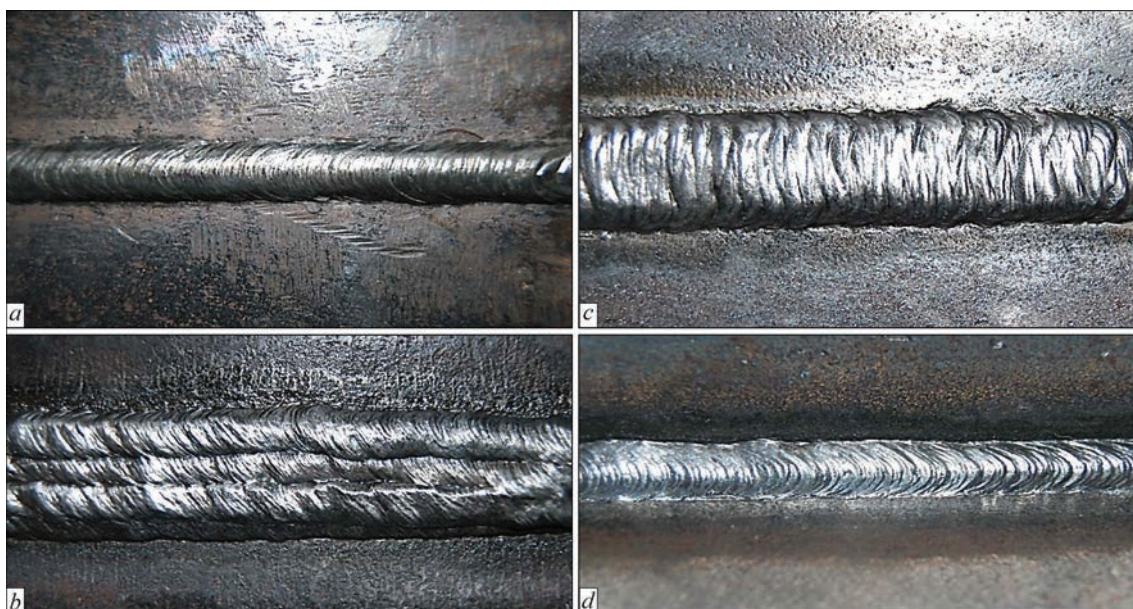
Figure 2. Appearance of butt ( a–c ) and fillet ( d ) welds in spatial positions: a — flat; b — horizontal; c — overhead; d — horizontal overhead
